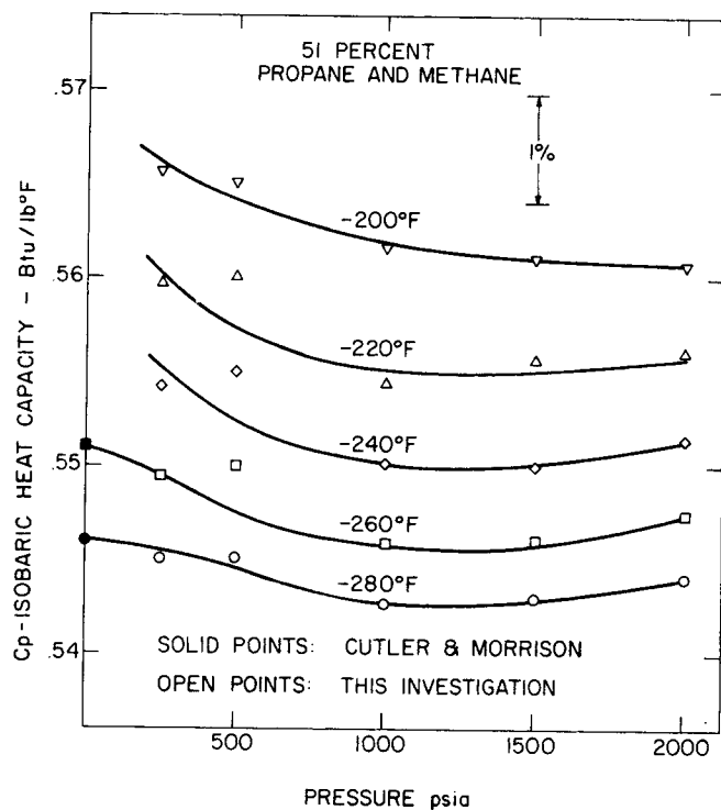
Fig. 10. The effect of pressure on C_p at low temperatures including comparison with data of Cutler and Morrison (5).
