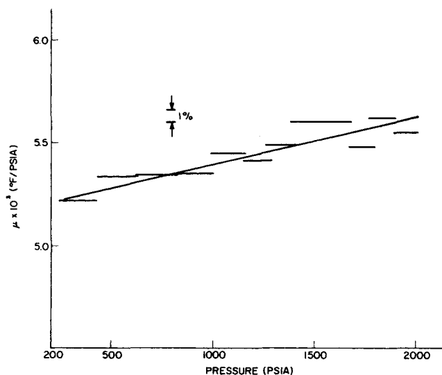
Fig. 8. Joule-Thomson coefficient at -149.0 °F.
